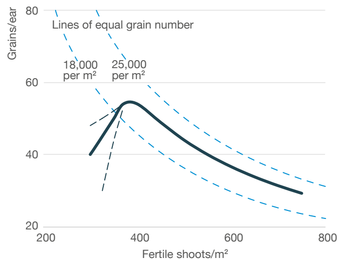
Figure 26. Grain numbers in the ears can compensate above 400 shoots/m 2
